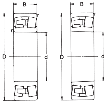
222R 圓柱孔
